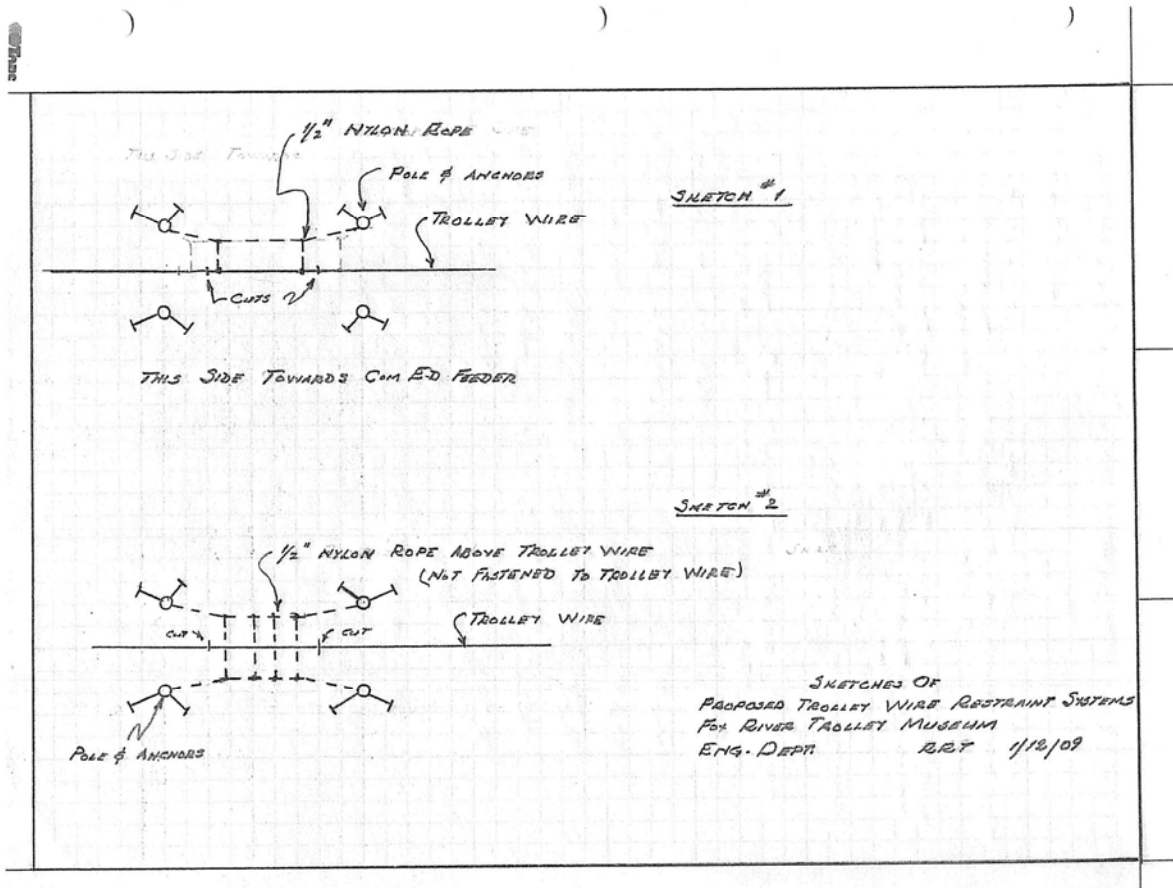
Figure 10 - Fox River Trolley Museum Trolley Wire Restraint Systems
